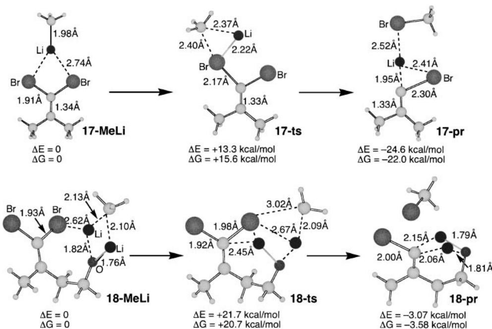
Fig. 2. Transition structures for the lithium-bromine exchange reaction [B3LYP/6-31+G(d)]. \Delta E and \Delta G are the differences in energy and the Gibbs free energy at 298.15 K, respectively.
