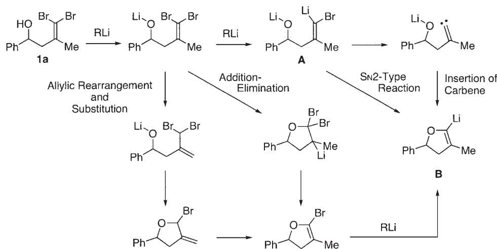
Scheme 4. Four possible mechanisms.
