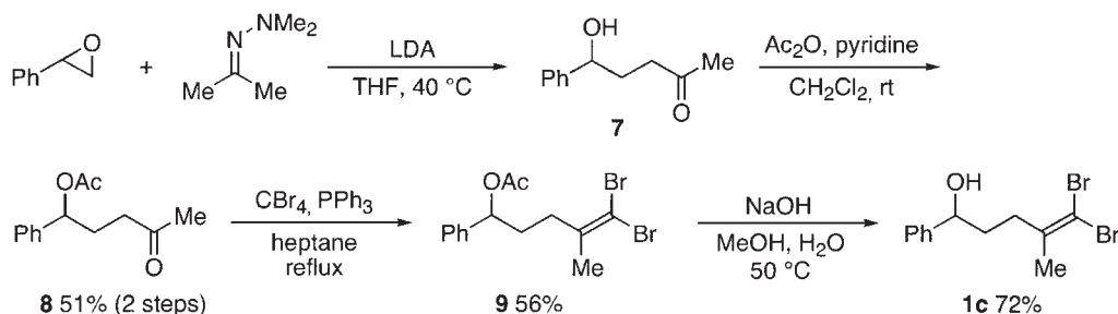
Scheme 2. Preparation of gem -dibromoalkenol 1c .
