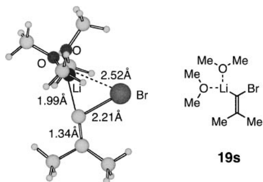
Fig. 3. The optimized structure of 19s [B3LYP/6-31+G(d)].
