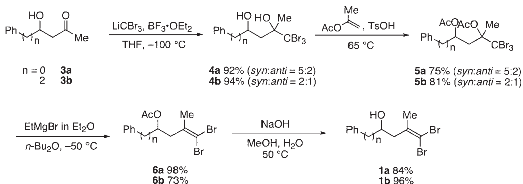
Scheme 1. Preparation of gem -dibromoalkenols 1a and 1b .
