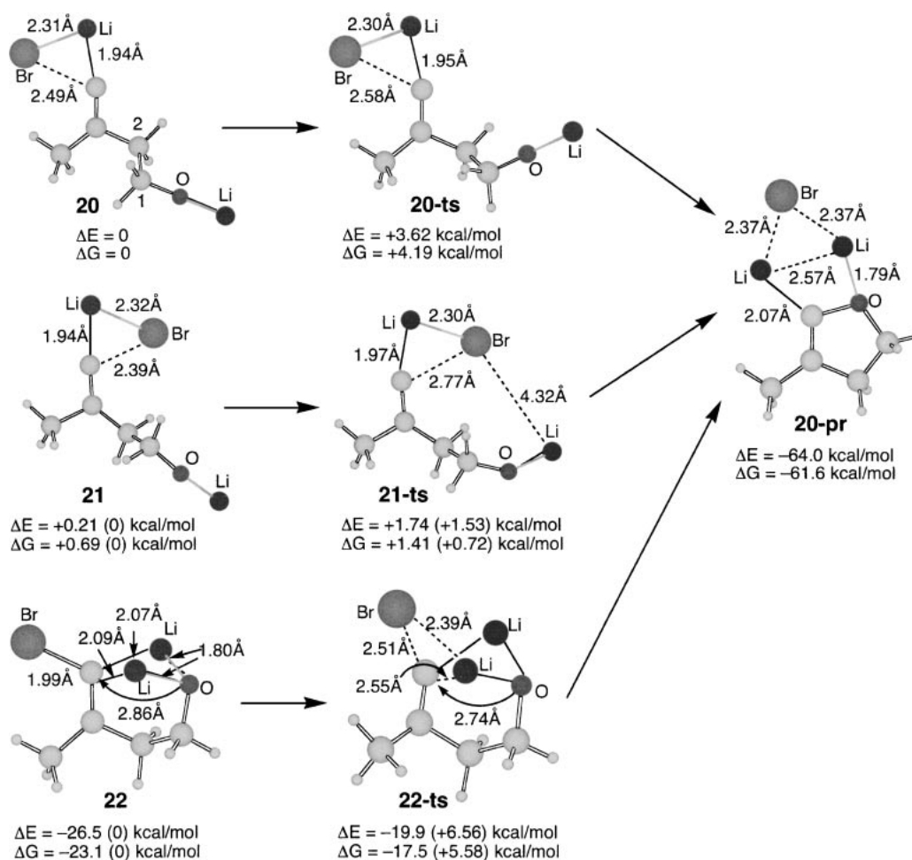
Fig. 4. Transition structures for the intramolecular substitution reaction of lithium alkylidene carbenoids [B3LYP/6-31+G(d)]. \Delta E and \Delta G are the differences in energy and the Gibbs free energy at 298.15 K, respectively.
