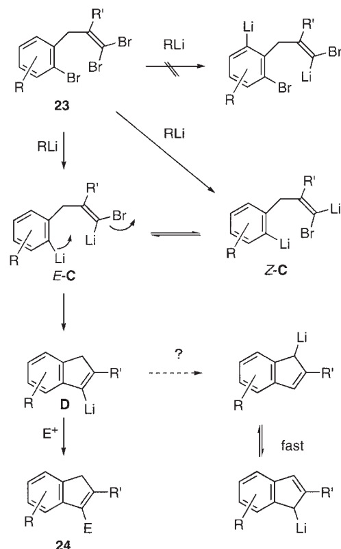
Scheme 6. Synthetic plan of indenenes 24 .
