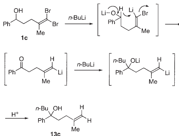
Scheme 3. Formation of alcohol 13c .
