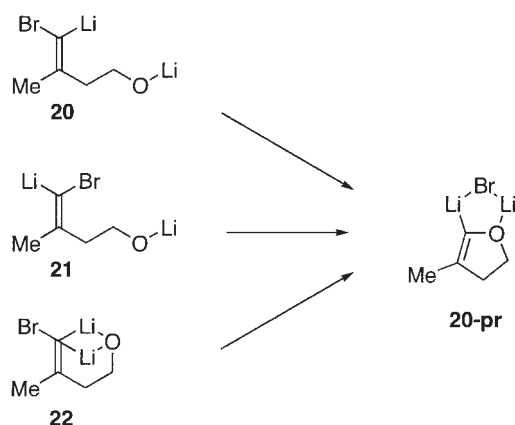
Scheme 5.
